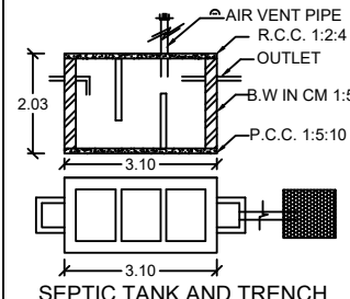
SEPTIC TANK AND TRENCH
