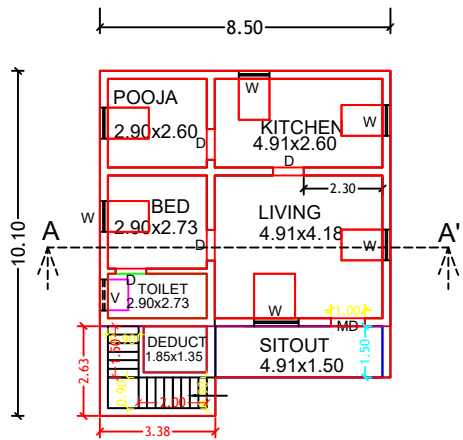
PROPOSE GROUND FLOOR PLAN
