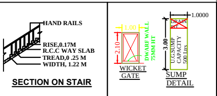
SUMP DETAIL
