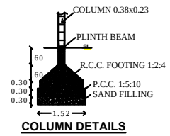
COLUMN DETAILS
