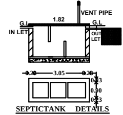
SEPTICTANK DETAILS
