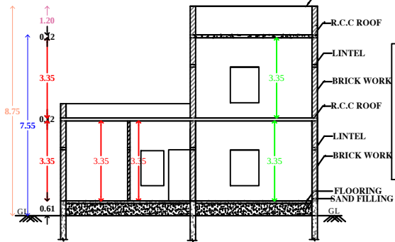
"SECTION "AB"
