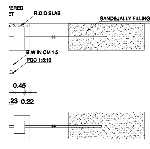
PLAN & SECTION OF SEPTIC TANK TRENCH
