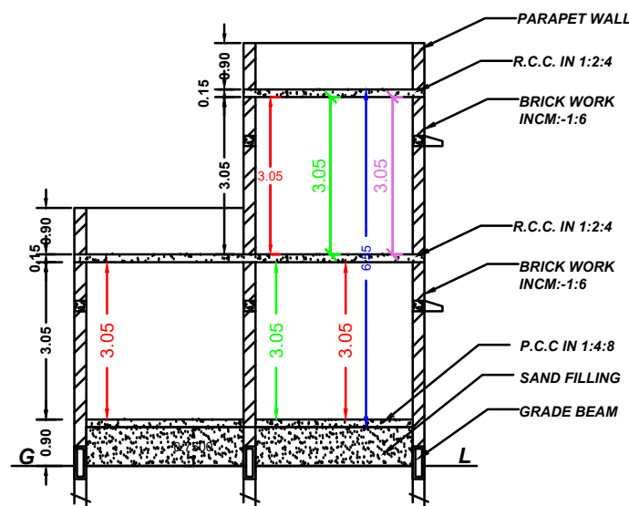
SECTION "AB"
