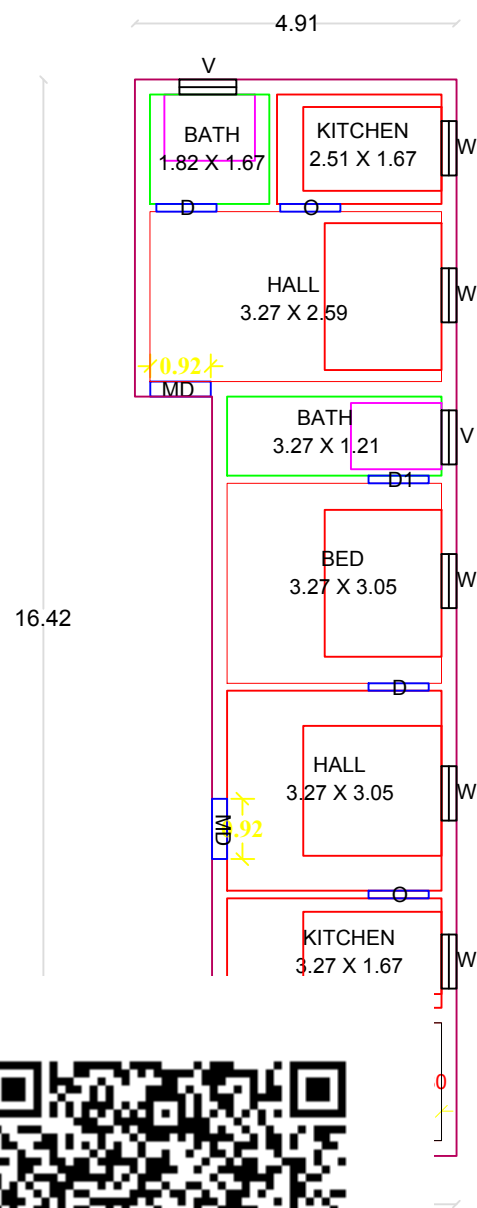
PLAN
