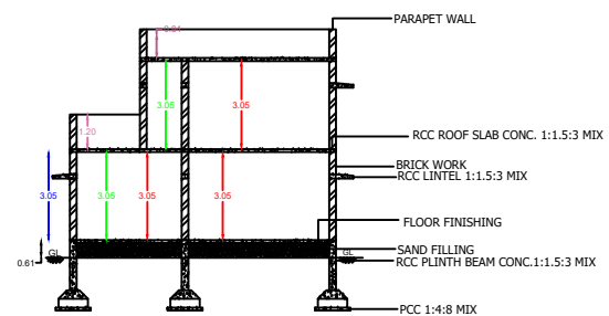
SECTION AB
