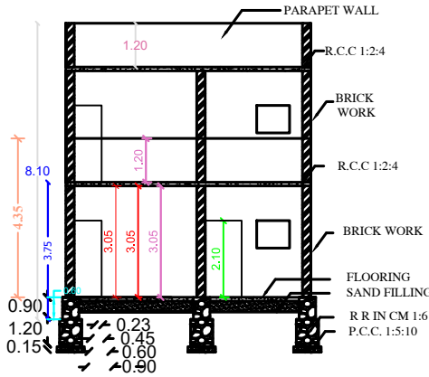
SECTION AB
