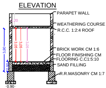
SECTION ON SV
