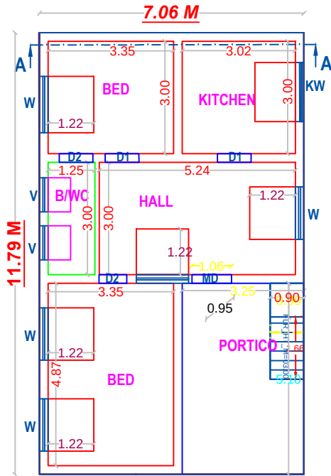
PLAN - GROUND FLOOR (PROPOSED)
