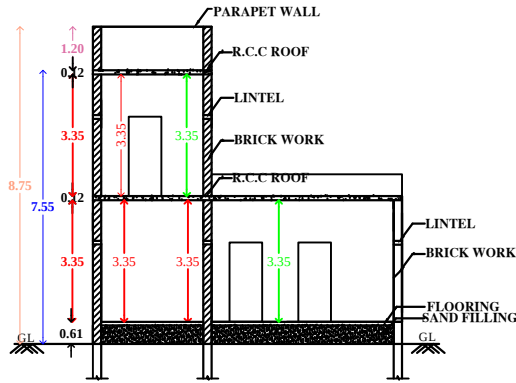
"SECTION "AB"
