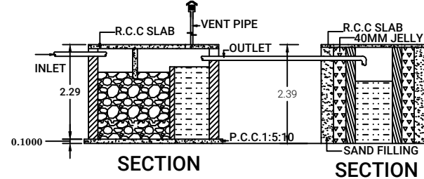
1000 GALLONS CAPACITY SEPTIC TANK (NTS)
