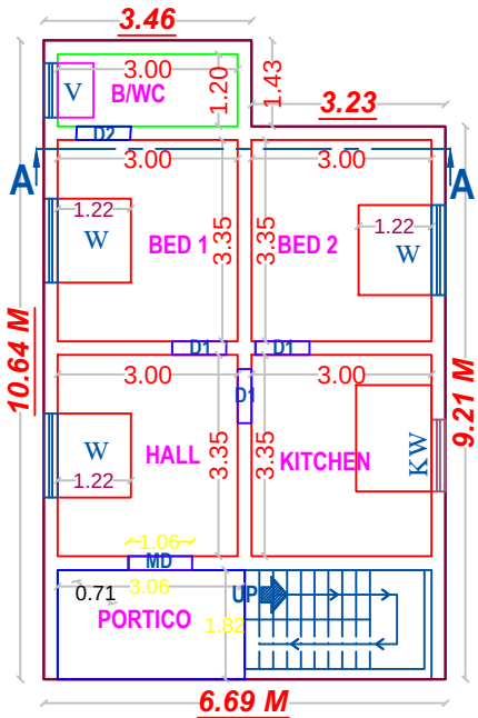
PLAN - GROUND FLOOR (PROPOSED)
