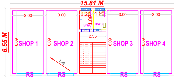
PLAN - GROUND FLOOR ( PRO.BUILDING )
