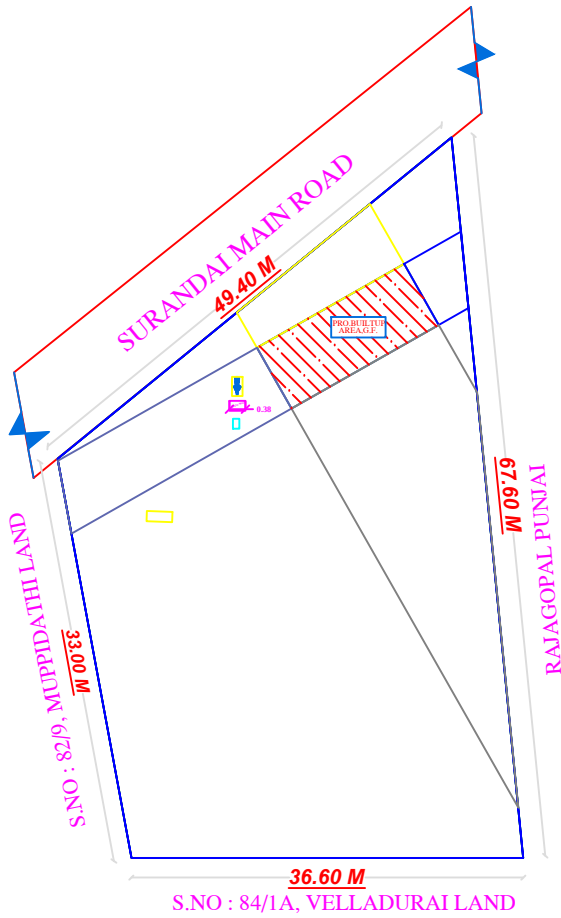
SITE PLAN SCALE:- 1:400
