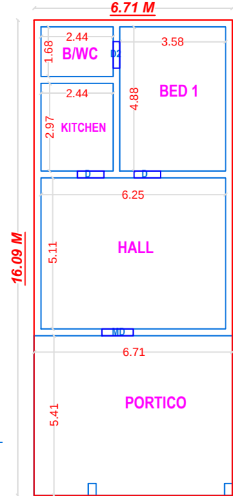
PLAN - GROUND FLOOR ( EXG.BUILDING )
