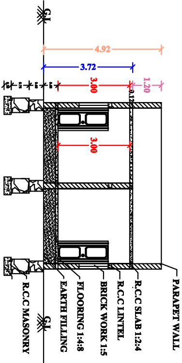
"SECTION "AB"
