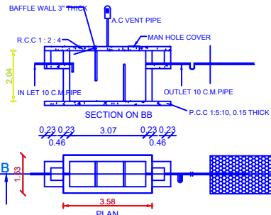
SEPTIC TANK AND TRENCH & U TRAP ADOPTED
