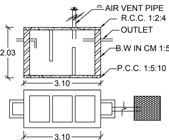
SEPTIC TANK AND TRENCH
