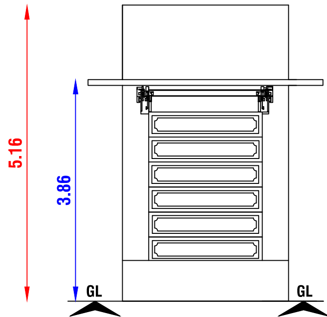
FRONT ELEVATION
