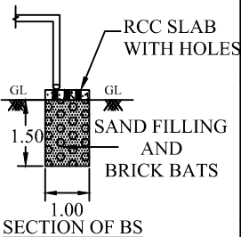
SECTION OF BS
