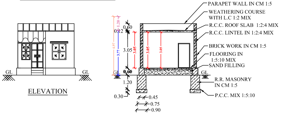
SECTION OF "AB"
