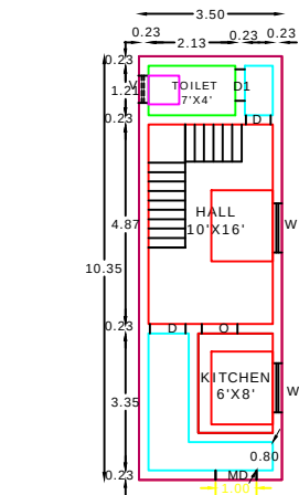
EXT GROUND FLOOR RESIDENTIAL PLAN
