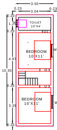
PRO FIRST FLOOR RESIDENTIAL PLAN
