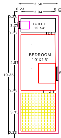
PRO SECONT FLOOR RESIDENTIAL PLAN
