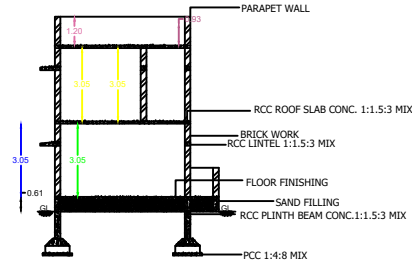
SECTION AB
