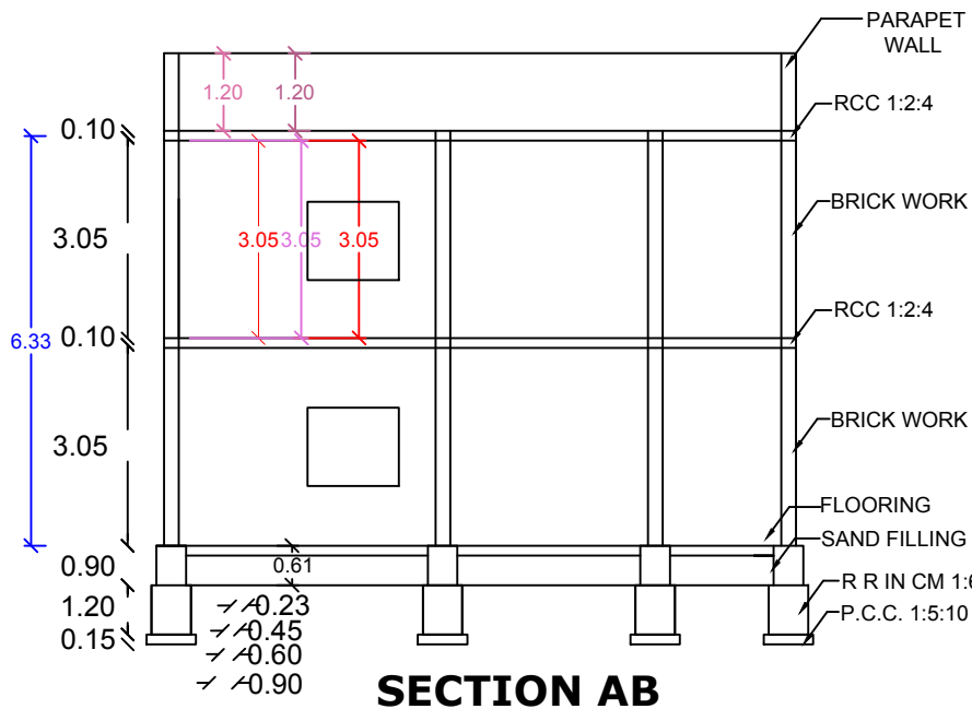
SECTION AB
