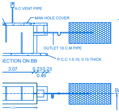
SEPTIC TANK AND TRENCH & U TRAP ADOPTED
