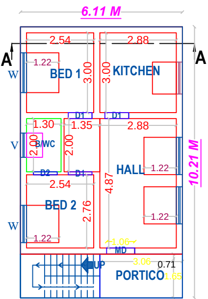
PLAN - GROUND FLOOR ( PROPOSED - 671.45 SQ.FT )
