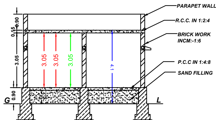
SECTION "AB"
