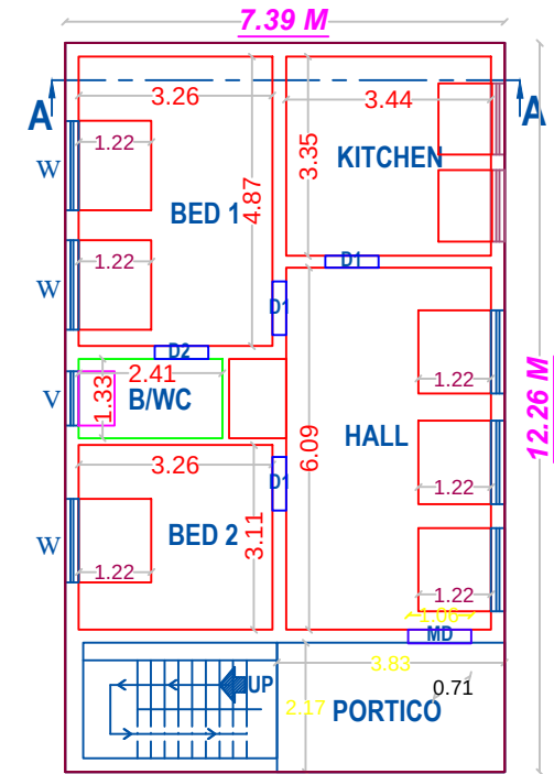
PLAN - GROUND FLOOR (PROPOSED)
