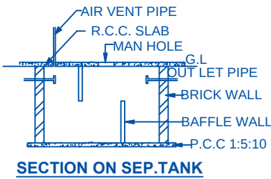
SECTION ON SEP.TANK
