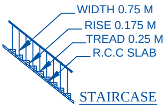
STAIRCASE
