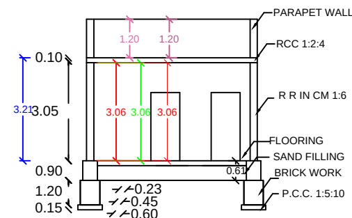
SECTION AB
