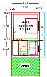
PRO FIRST FLOOR RESIDENTIAL PLAN
