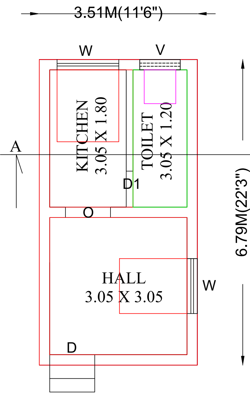
PLAN
