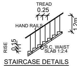
STAIRCASE DETAILS
