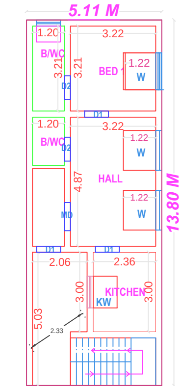
PLAN - GROUND FLOOR (PROPOSED)
