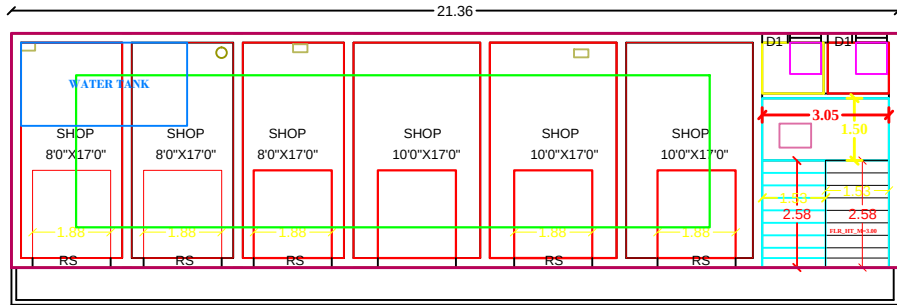
PRO.FIRST FLOOR PLAN
