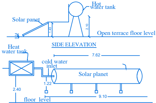
SOLAR WATER HEATER PLANT
