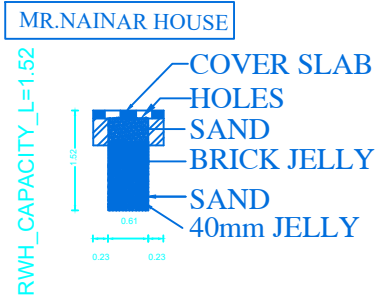
SECTION OF RAIN WATER COLLECTION TANK
