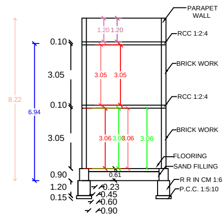
SECTION AB
