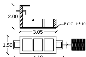
4.18 SEPTIC TANK AND TRENCH
