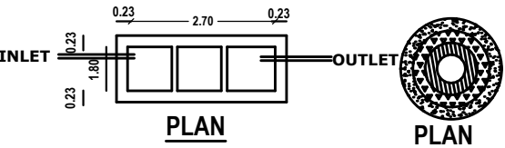
SEPTICTANK DETAILS
