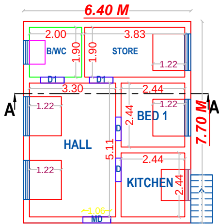
PLAN - GROUND FLOOR (PROPOSED - 530.44 SQ.FT)
