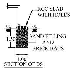
SECTION OF BS
