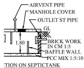
SECTION ON SEPTICTANK
