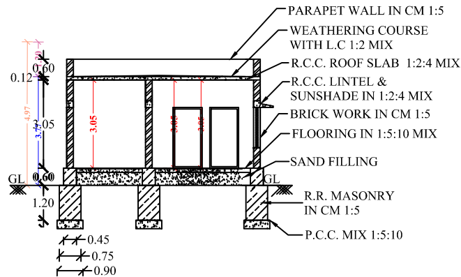
SECTION OF "BS"
