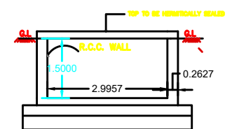
RWH SECTION
