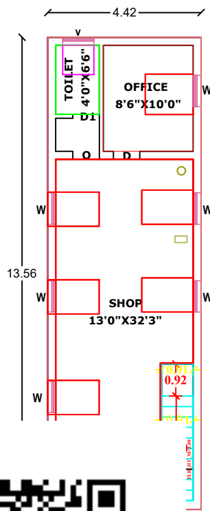
R PLAN
