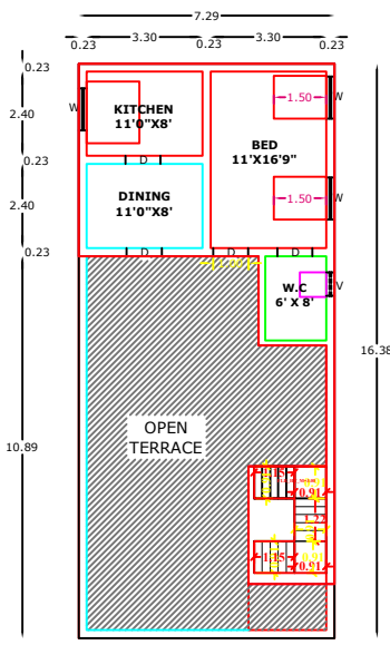
FIRST FLOOR RESIDENTIAL PLAN
