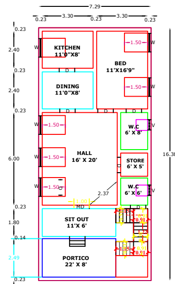
GROUND FLOOR RESIDENTIAL PLAN
