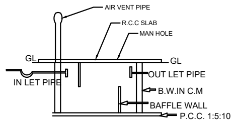
SECTION ON SEPTIC TANK
