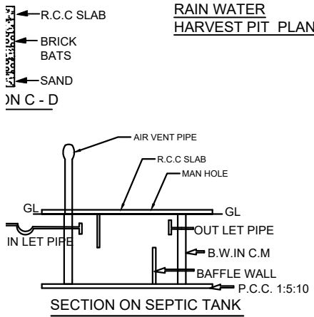
SECTION ON SEPTIC TANK
