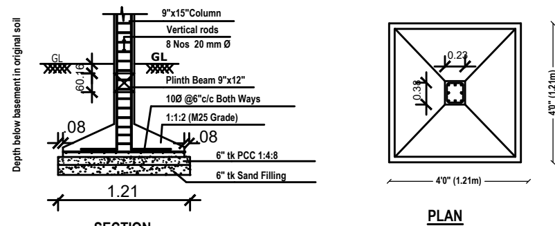
COLUMN FOOTING DETAILS
