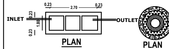
SEPTICTANK DETAILS
