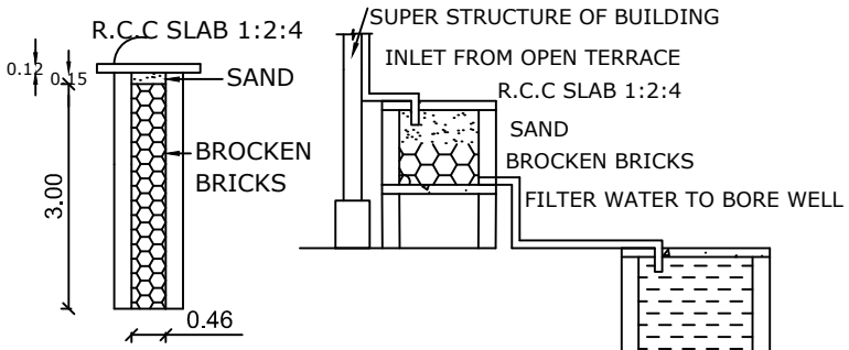
DETAILS OF FILTER BED & WELL
