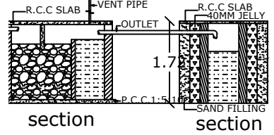
1000 GALLONS CAPACITY SEPTIC TANK (NTS)
