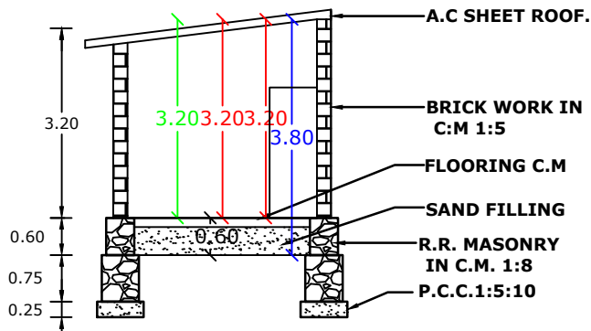
CROSS SECTION ON A-B
