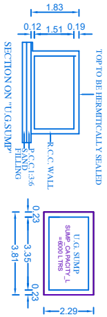
SITE PLAN
