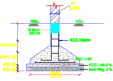
FOUNDATION DETAIL
