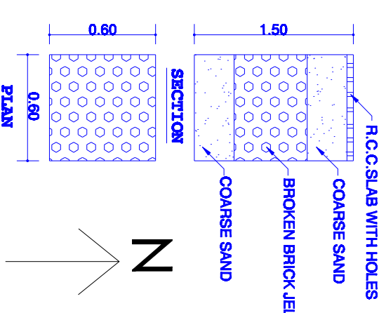
RAIN WATER HARVESTING WASTE WATER FROM WASH BASIN AND BATHROOM ARE RECHARGED AND RECYCLED AND TO BE CONNECTED WITH R.W.H. PT.
