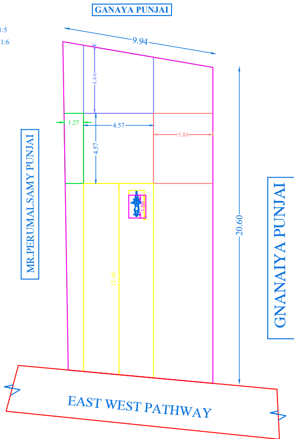
SITE PLAN
