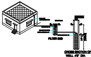
PRO.RAIN WATER SYSTEM
