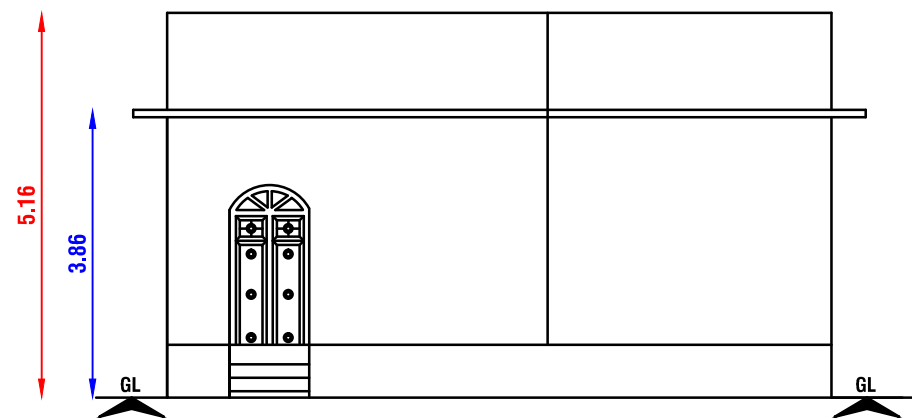
FRONT ELEVATION
